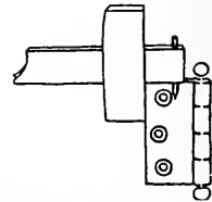
FIG. 451. SETTING GAGE FOR WIDTH OF GAIN.
